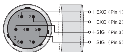
DBST-HK(30t/70t)
