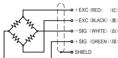
DBST-HK(100t)
