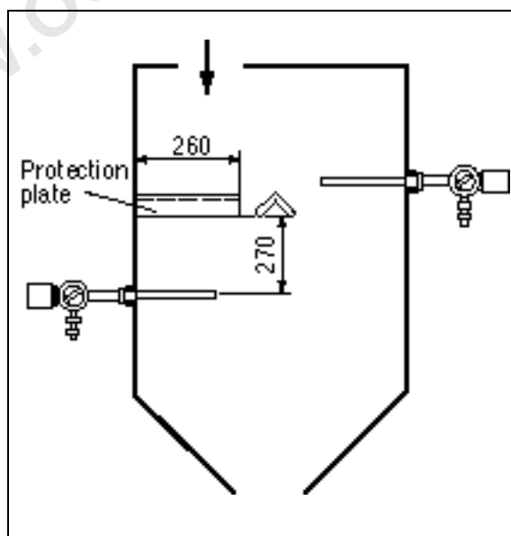
Fig. 1 Schematic diagram for installation
