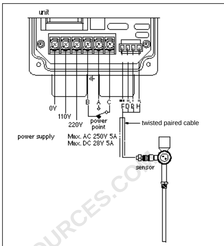
Fig. 2 Schematic diagram for wiring
