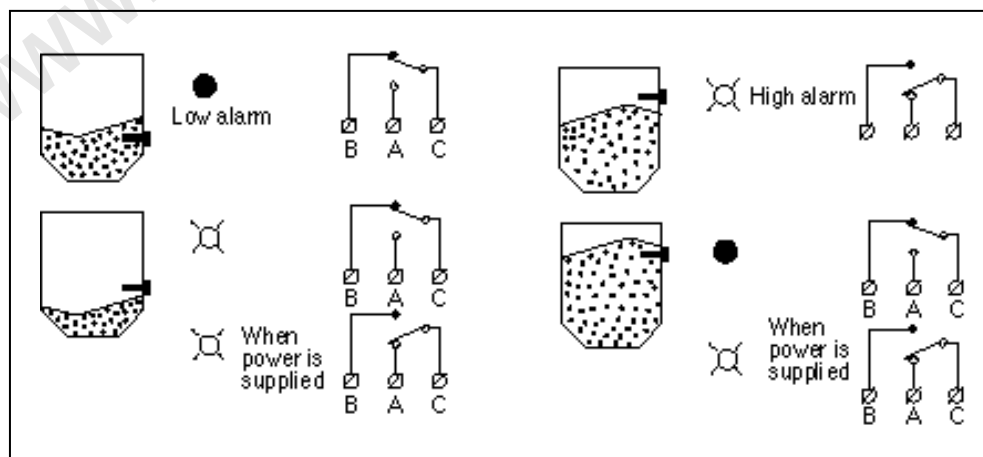
Fig. 3 LED and operation of contact point
